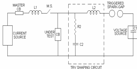
Fig.1. Synthetic testing circuit
