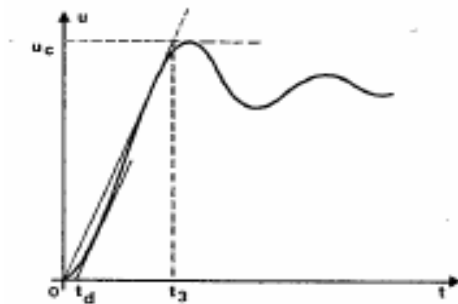
Fig.2 IEC envelope defined by 2Parameters: u_c and t_3
