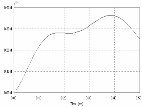
Fig. 9. TRV curve for 245 kV circuit breaker (for the simulated control circuit-II shown in fig. 5)
