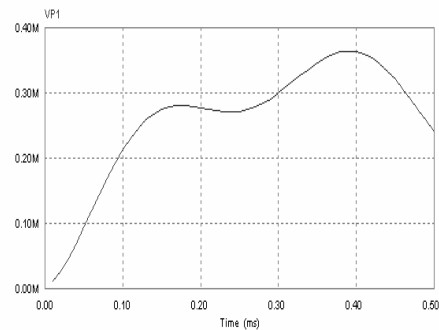
Fig.10. TRV curve for 245 kV circuit breaker (for the simulated control circuit- III shown in fig. 6)
