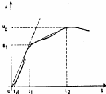
Fig.3 IEC envelope defined by 4- Parameters: u_1 and t_1, u_c and t_2
