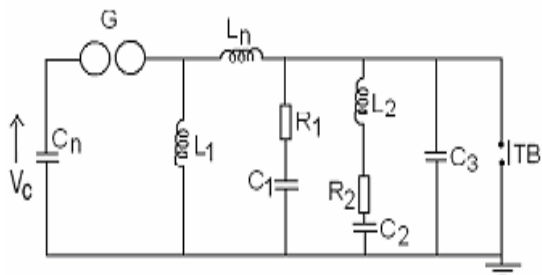
Fig. 5. 4 parameters TRV synthetic testing control circuit II
