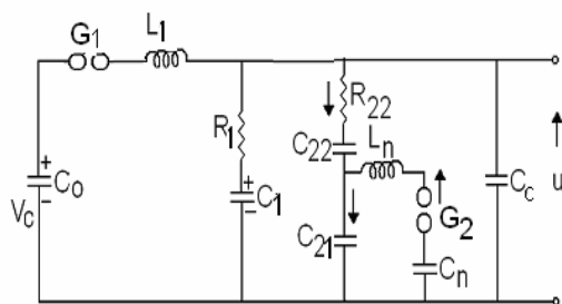
Fig. 6. 4 parameters TRV synthetic testing control circuit III
