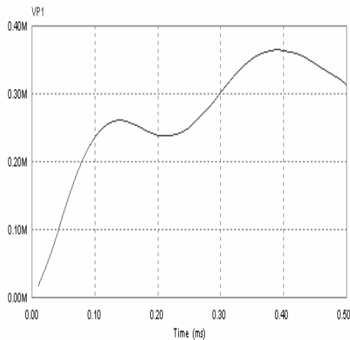
Fig. 8. TRV curve for 245 kV circuit breaker (for the simulated control circuit-I shown in fig. 4)
