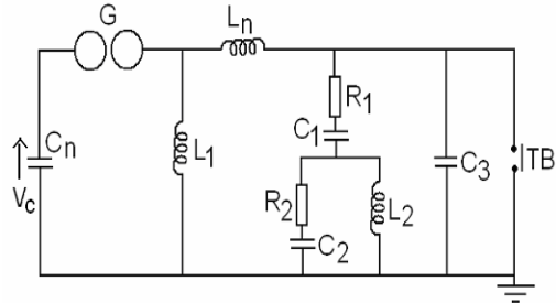
Fig. 4 4 parameters TRV synthetic testing control circuit I
