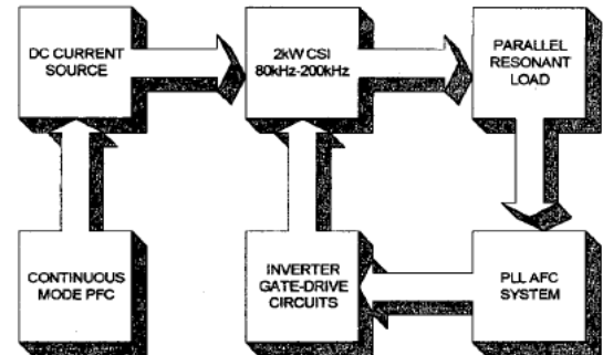
Fig. 1. Block diagram configuration.
