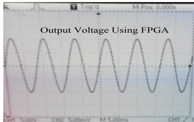
Fig. 10. Output Voltage Waveform Using FPGA Controller
