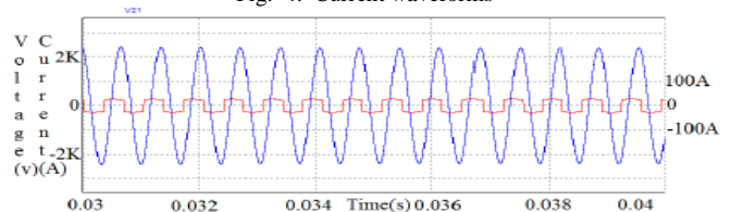
Fig. 4. Current waveforms
