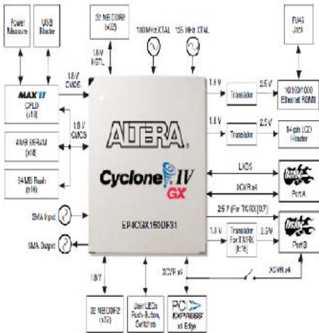
Fig. 9. FPGA controller
