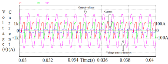
Fig. 6. Voltage and Current waveforms
