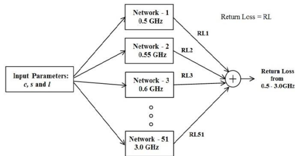
Fig 3: Proposed ANFIS architecture
