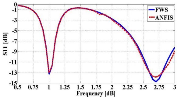
Fig 5: Comparison of return loss for a= 11.5\text{mm} , l_f= 21.5\text{mm} and d= 4.5\text{mm}
