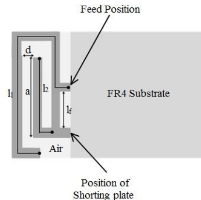
Fig 1: Schematic of hexa-band PIFA under consideration
