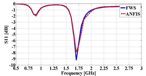
Fig 5: Comparison of return loss for a=1.5\text{mm} , l_f=1.5\text{mm} and d=1.5\text{mm}
